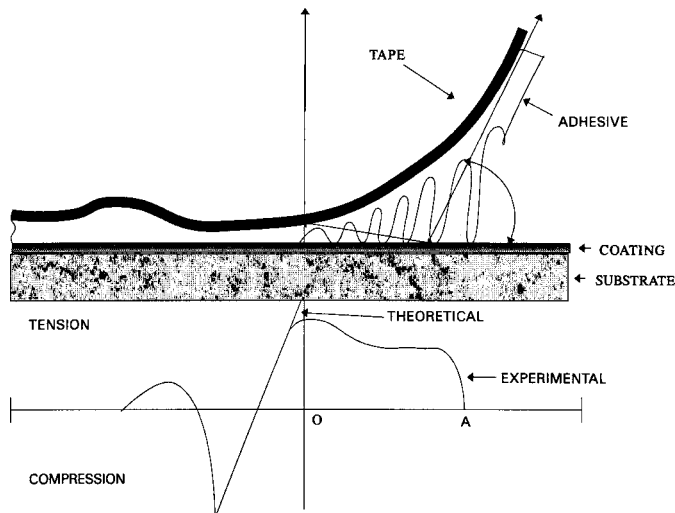
FIG. X1.1 Peel Profile (6)
